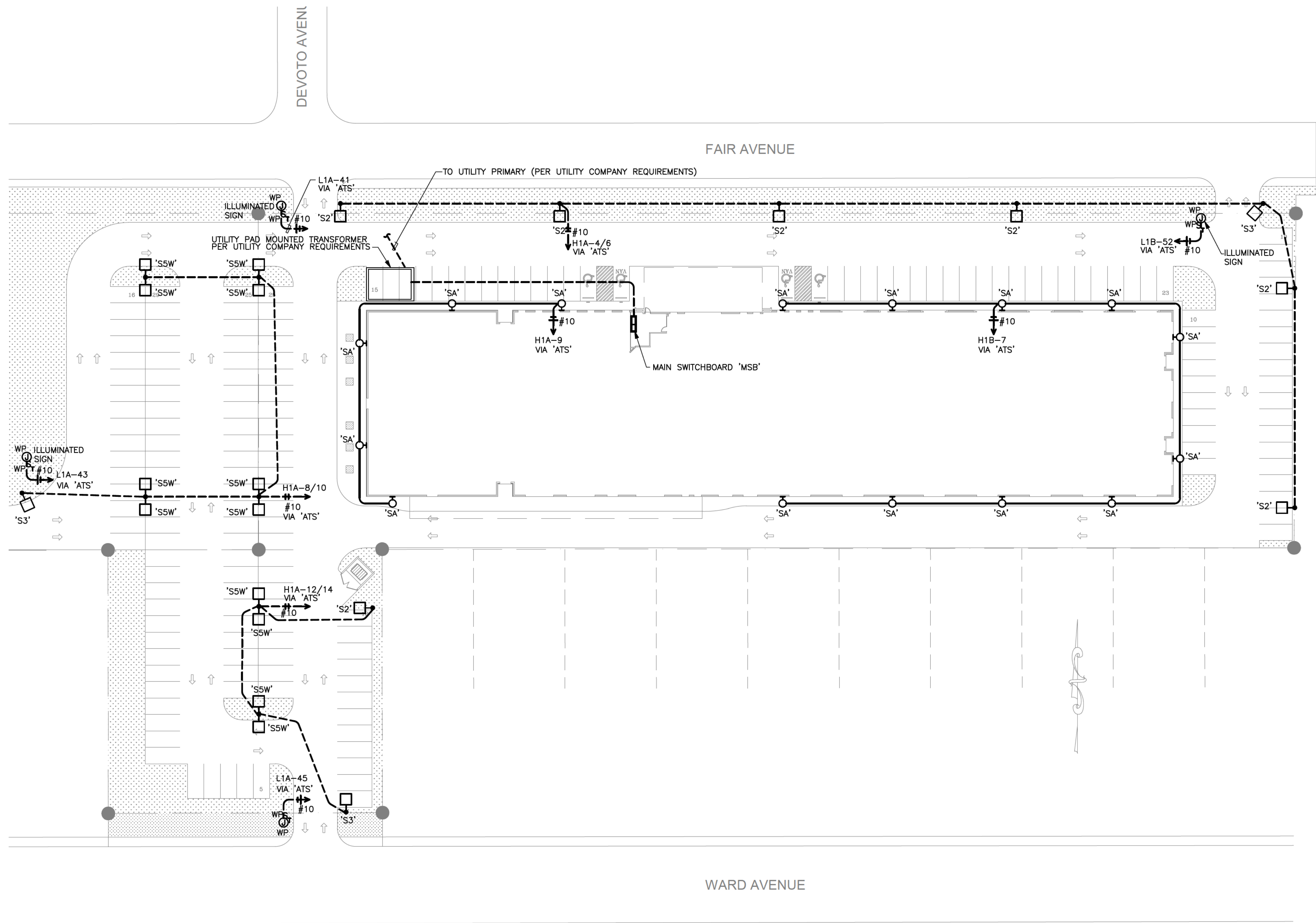
1 ELECTRICAL SITE PLAN SCALE: 1/32"=1'-0"
